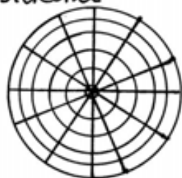
stereonet
