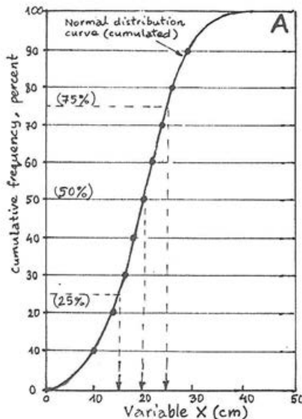
Fig. 5. Cumulative frequency of grouped data plotted in arithmetic (A) and probability scale (B) on the percentage axis. Normal frequency distribution is a straight line when plotted in probability scale (B). Note that a whole range of percentiles can be read from the curve to characterize the shape of the frequency distribution; the 50th percentile, X_{50} , is called "median".
