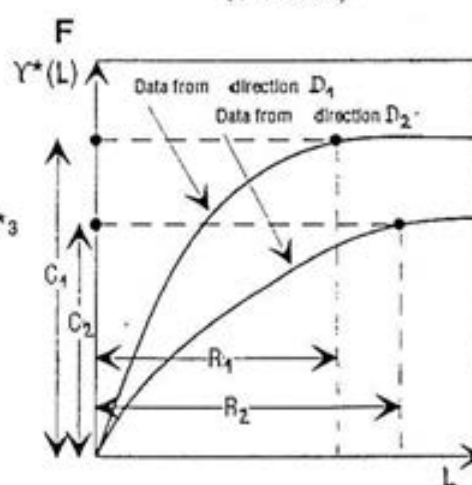
Anisotropy model (spherical-type example)
