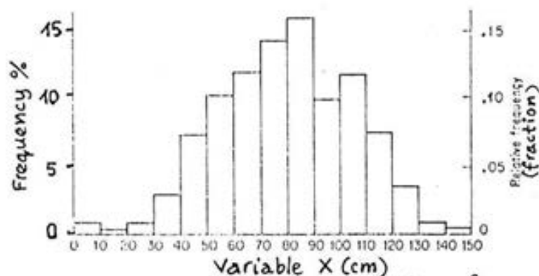
Fig. 2. The grouped data set presented as frequency histogram.
