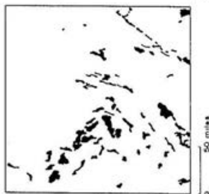
FIGURE 5.82 Locations of major oil and gas fields in central Kansas.
