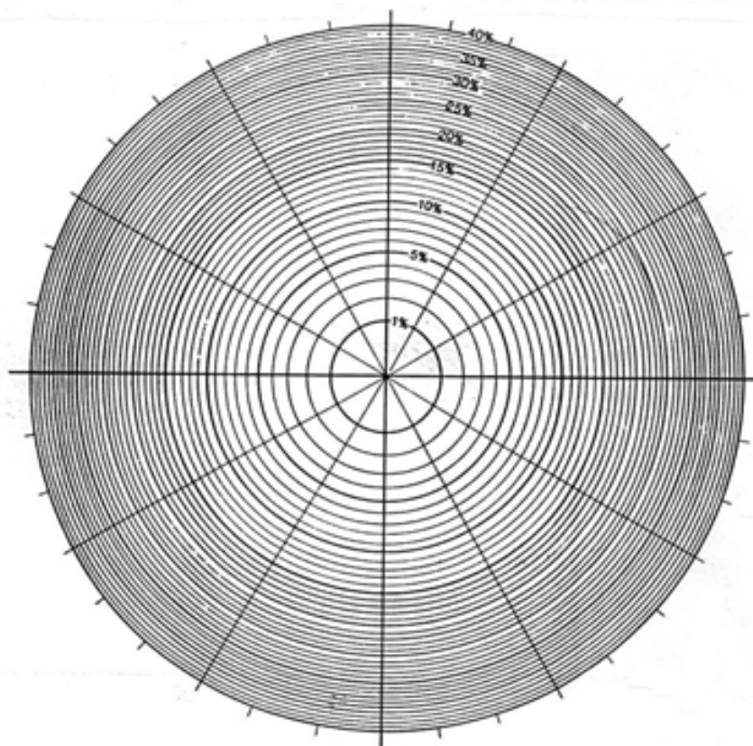
Fig. 3. A frequency net produced to facilitate rapid construction of circular histograms. The net (frequency circles) can be extended to higher values, if needed, with the use of formula (1) given in text; r_{1\%} = 8 mm in the present case. The % symbols have to be omitted if pure number frequencies (not percentages) are plotted.
