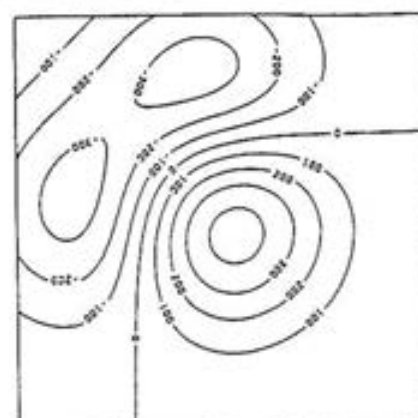
Fig. 3. The synthetic surface computed from the regular grid. The amplitude of this surface is about 800 units.
