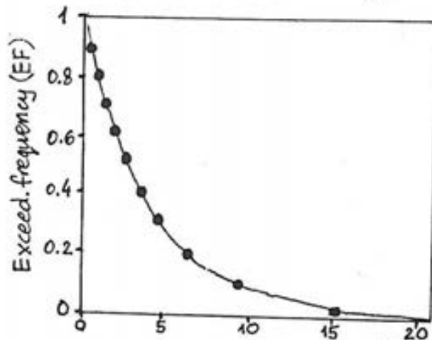
Fig. 10. A sample population of 10 beds with thicknesses, x_i (in cm), listed from the thinnest to the thickest (table). Nine of the 10 beds are thicker than the thinnest bed ( EF=0.9 ), eight of 10 are thicker than the next thinnest ( EF=0.8 ), seven of 10 are thicker than the next ( EF=0.7 ), etc.
