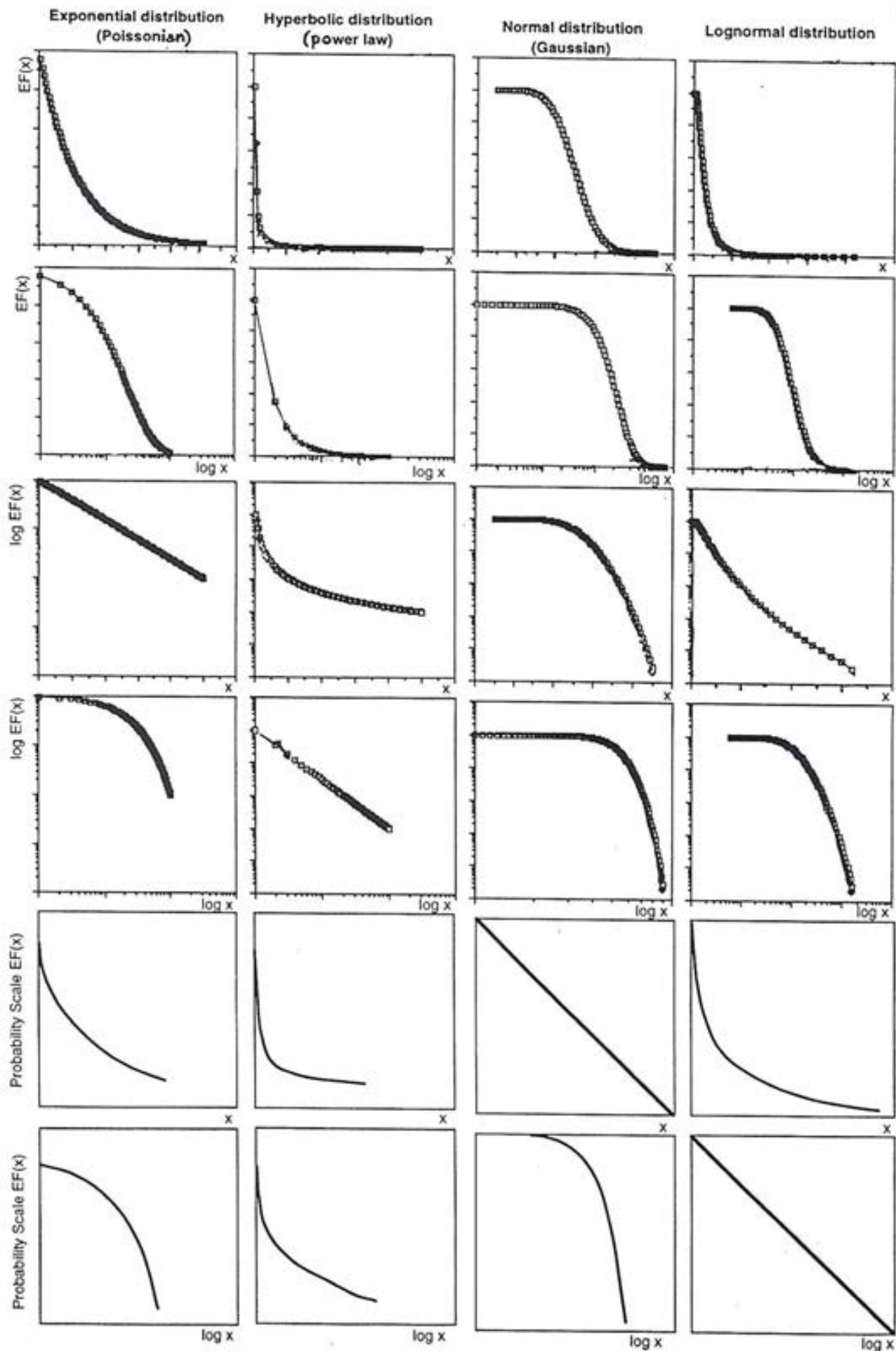
Fig. 12. Exceedance frequency (EF) plots of four common types of data distribution in different scales - a guide to the recognition of distribution type.
