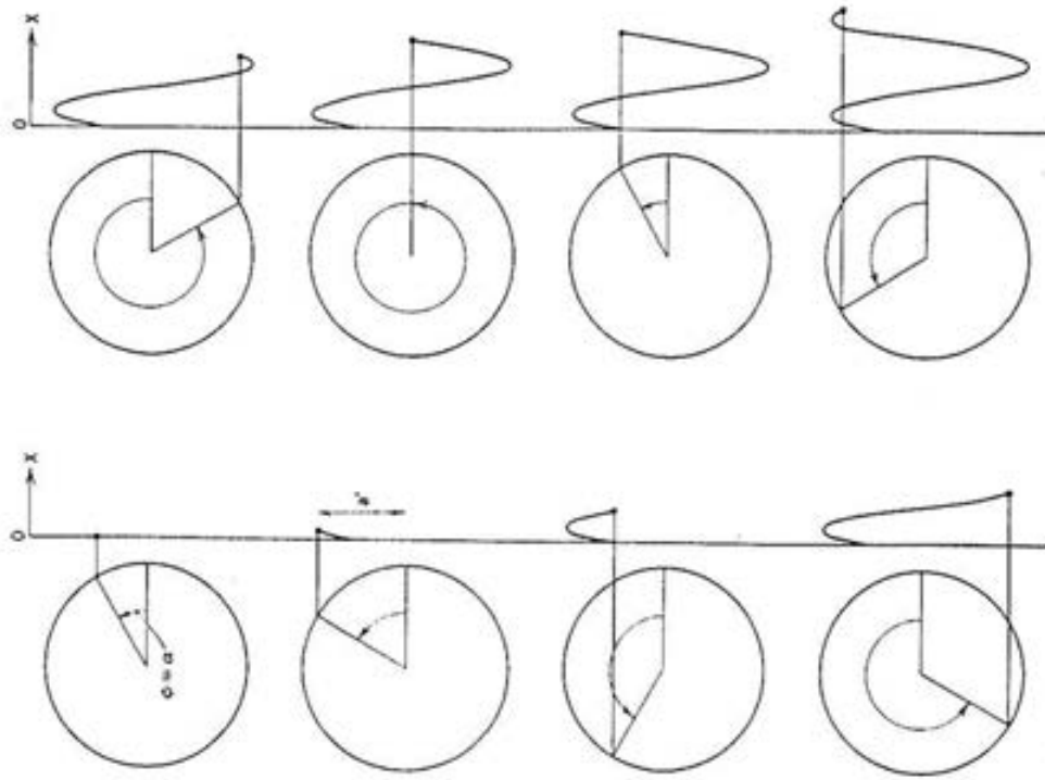
FIGURE 4.51 Progressive changes in phase angle from an initial value \phi . At successive values of x , Y = A \sin (2\pi x/X + \phi) and \alpha = (2\pi x/X + \phi) .
