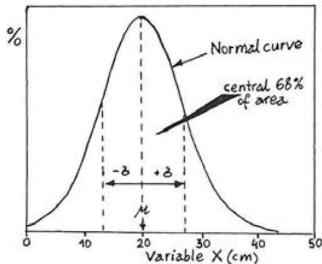
Fig. 6. The area under the frequency curve is called the distribution density; ca. 68% of the density is within the range of one standard deviation ( \pm \sigma ) around the mean ( \mu ), and nearly whole density is within the range of \pm 3\sigma around the mean. The mean value ( \mu ) defines the distribution central tendency, or the bell-shaped curve's central point.
