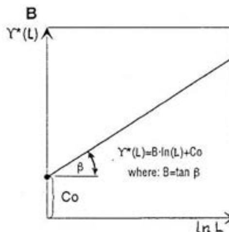
De Wijs's model (logarithmic)
