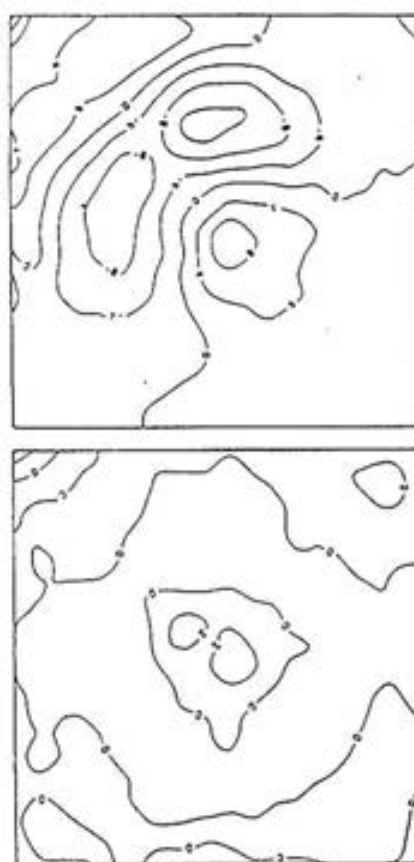
Fig. 4. Two maps of residuals obtained by polynomial interpolation from 400 data points show the effect of degree of the polynome. (a) (top) is obtained by a third degree polynomial interpolation; (b) is obtained by fourth degree.
