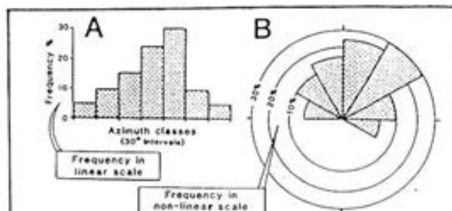
Fig. 1. Simple columnar histogram (A) and its circular equivalent (B). The diagrams, and their equivalent columns (A) and sectors (B), have the same areas. Note that the frequency scale becomes non-linear when histogram A is squeezed into a circular form B.
