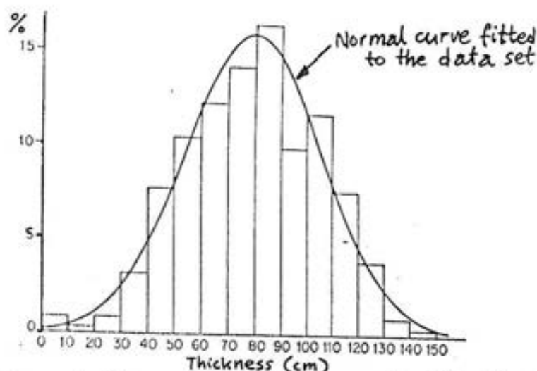
Fig. 3. Normal (Gaussian) curve approximating the histogram; vertical scale somewhat enlarged for visual purpose. The data set is the same as in Table 1 and Figs. 1-2.
